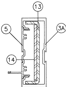
MULLION 'MD4'
