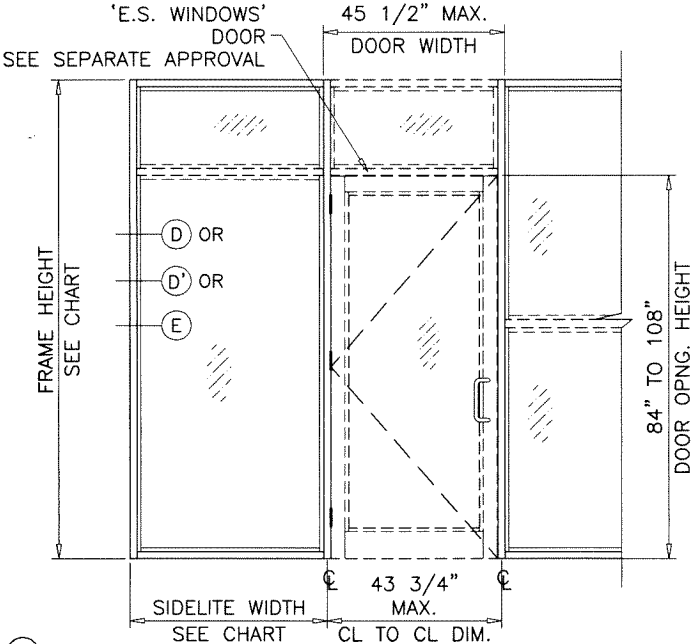
DOOR-WINDOW WALL TRANSITION MULLION
